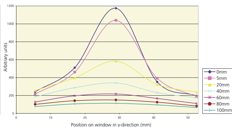
Intensity perpendicular to lamp axis (various distances)
