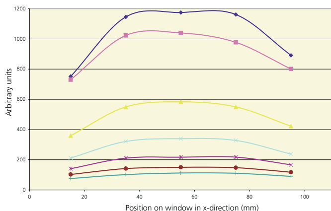
Intensity along lamp axis (various distances)
